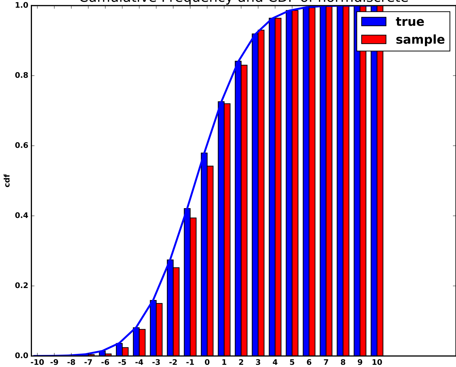
Cumulative Frequency and CDF of normdiscrete
