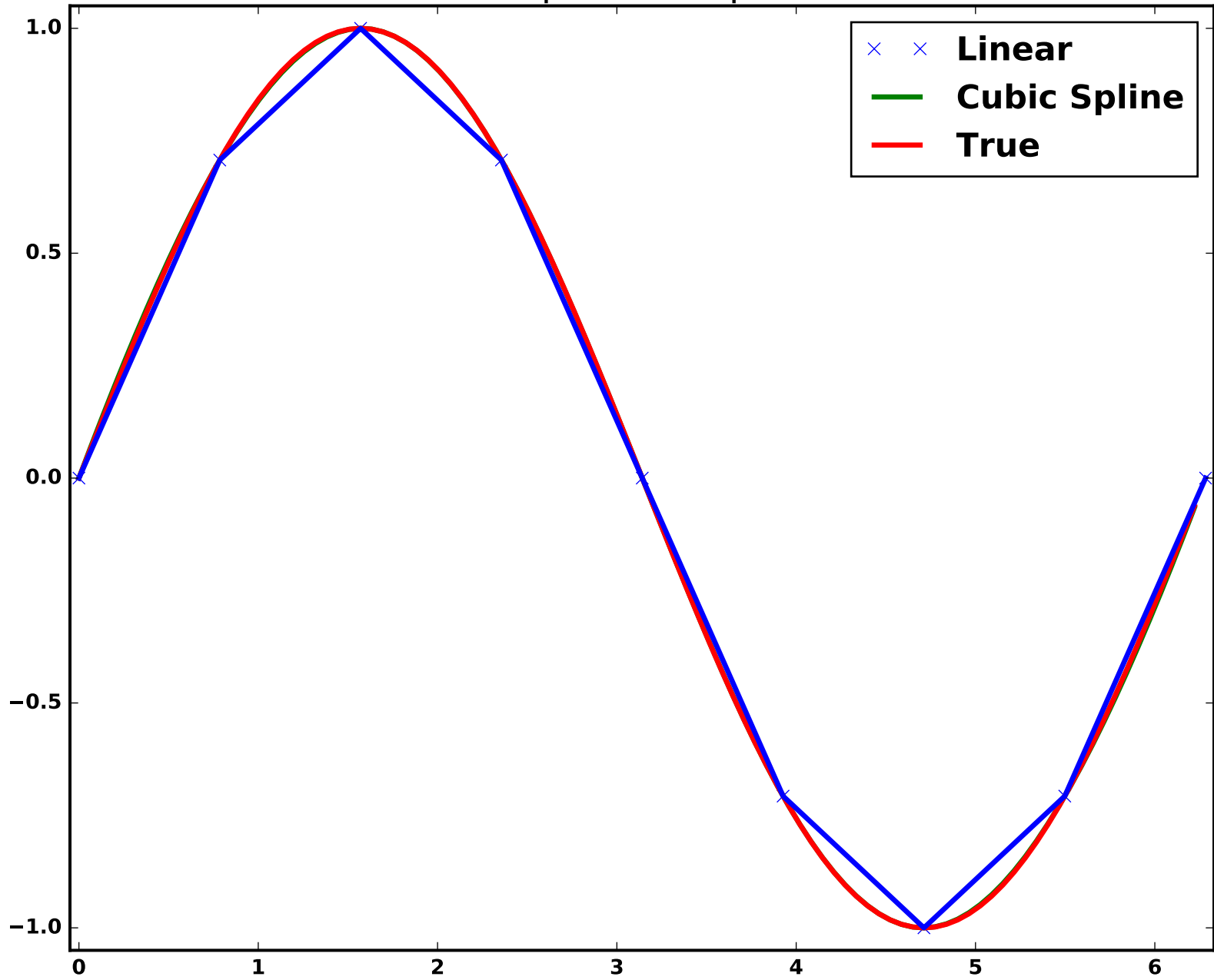
Cubic-spline interpolation
