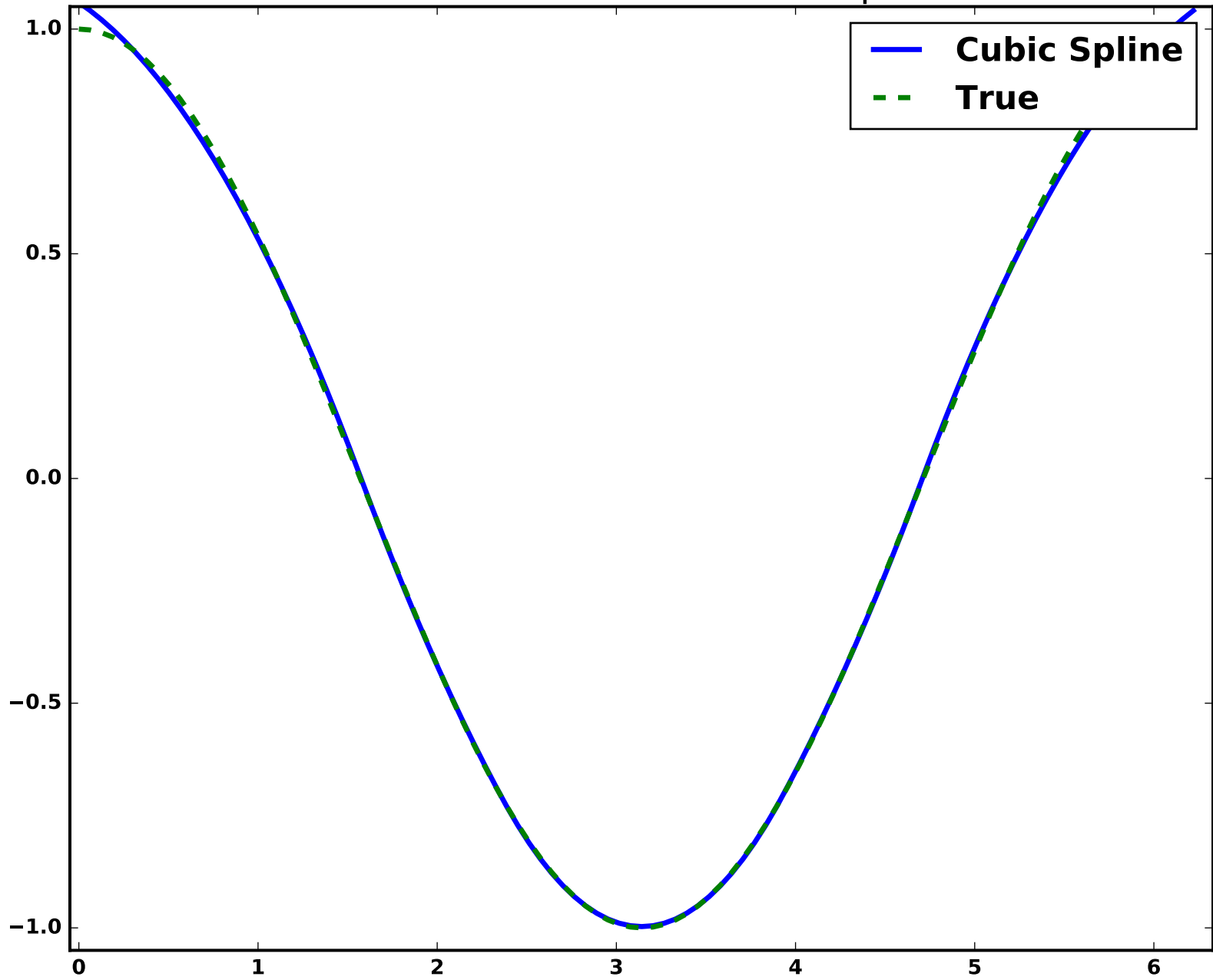
Derivative estimation from spline
