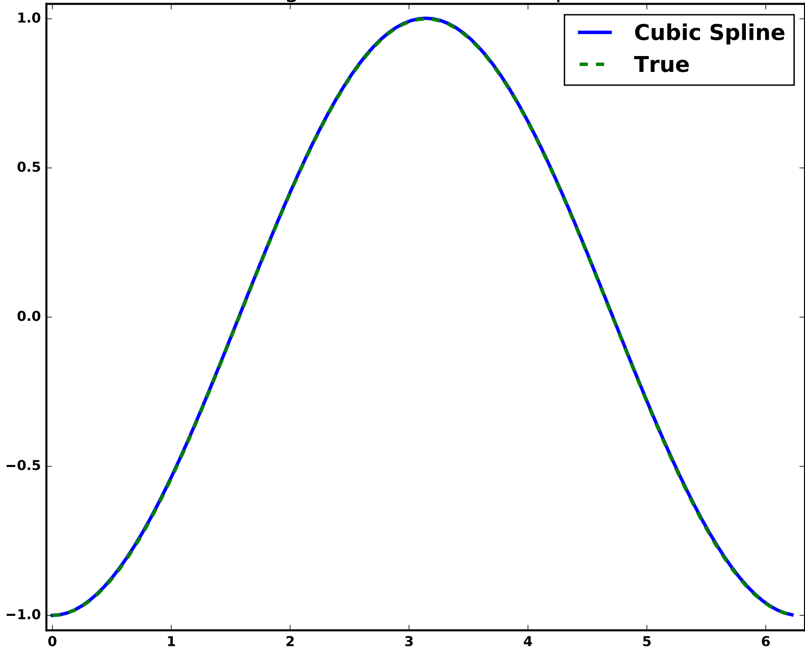
Integral estimation from spline
