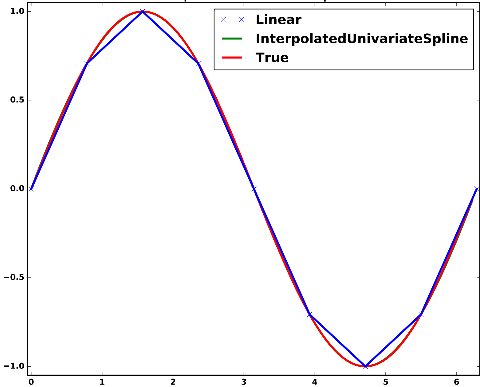
InterpolatedUnivariateSpline
