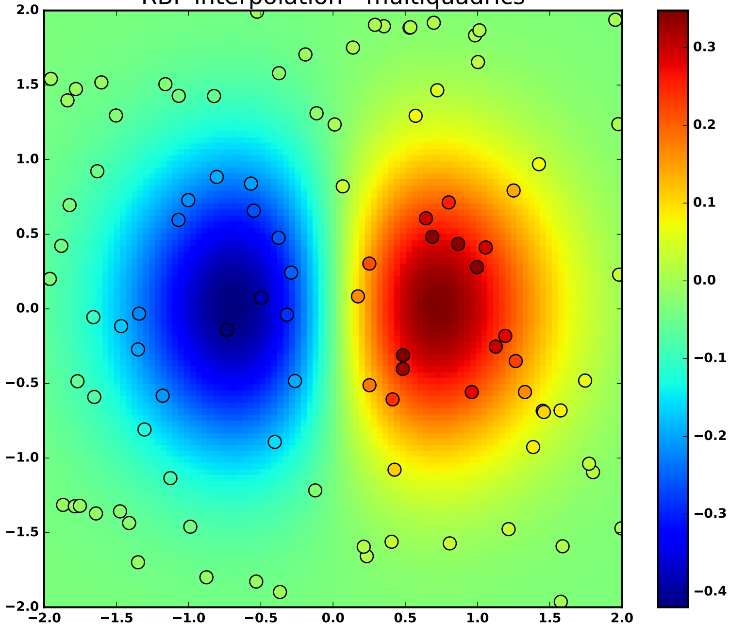
RBF interpolation - multiquadrics
