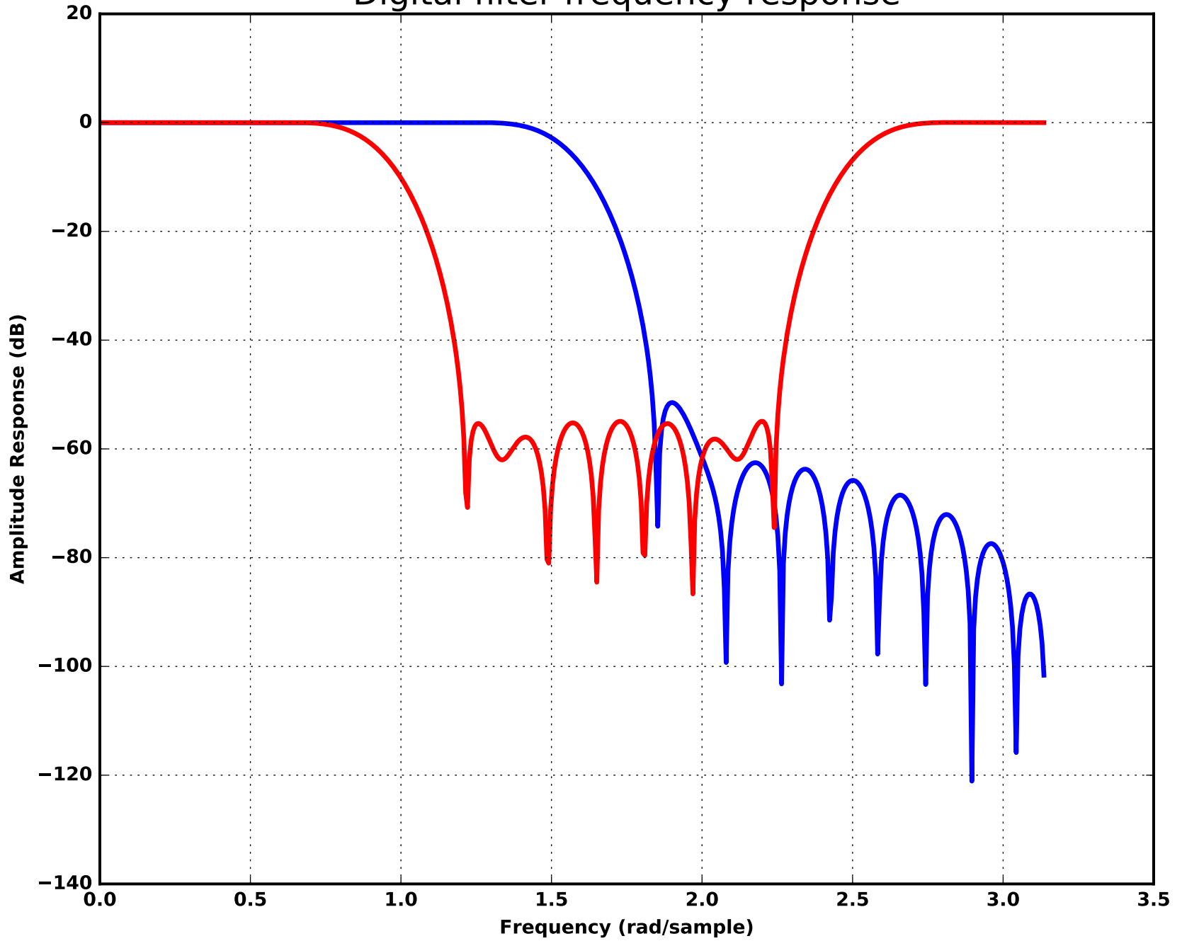
Digital filter frequency response
