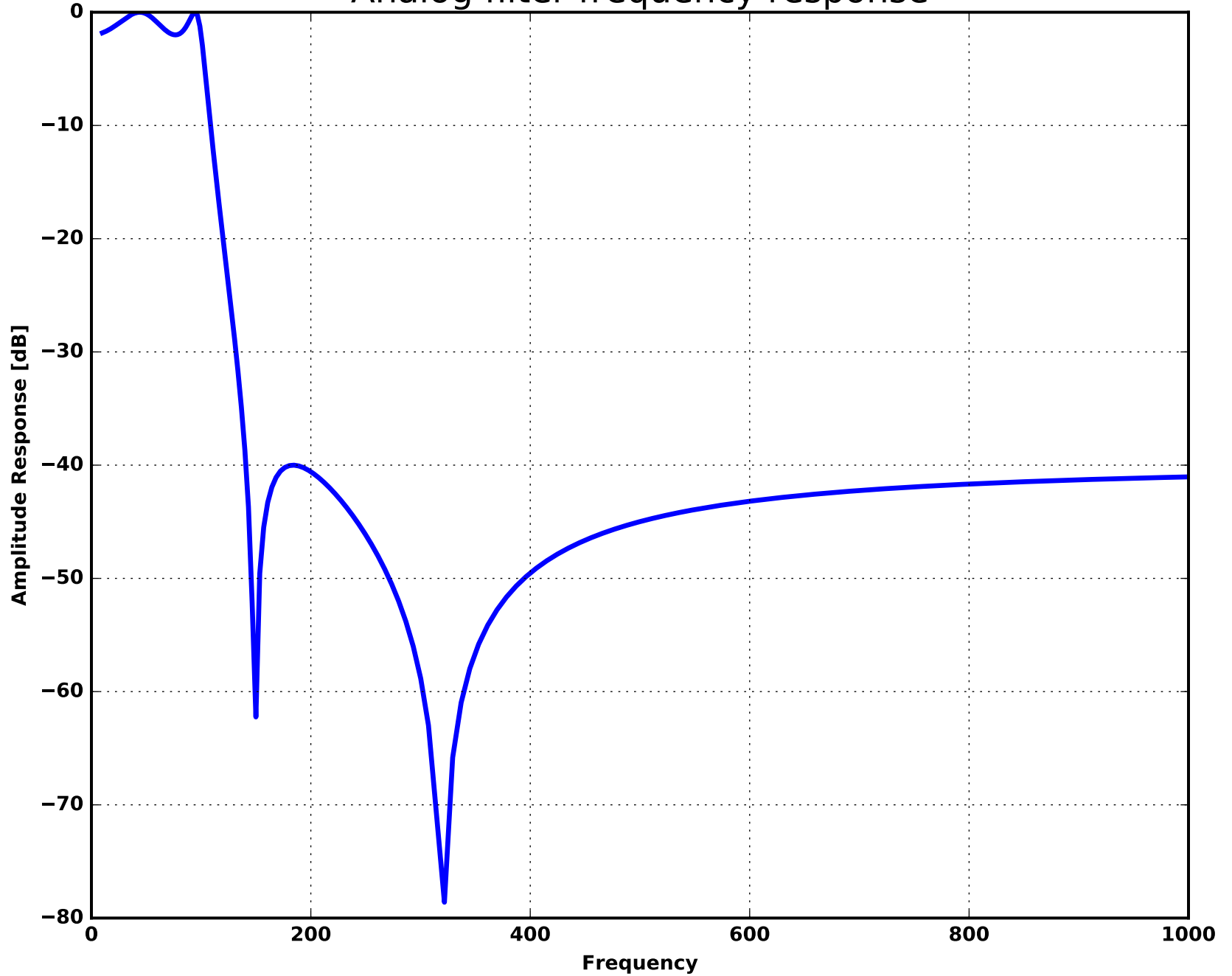
Analog filter frequency response
